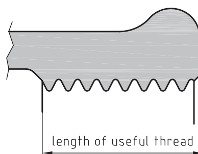
illustr. 5 Parallel internal thread Rp
