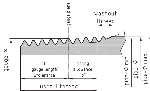
illustr. 3 Taper external thread R
