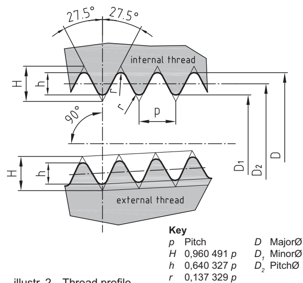
illustr. 2 Thread profile
