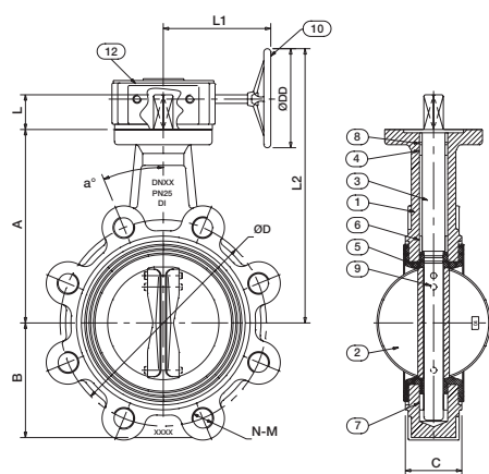
FM639 Gearbox Butterfly Valve
